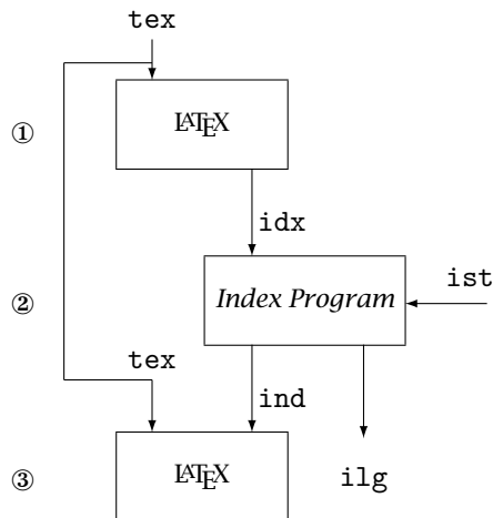
Figure 14.1: The sequential flow of index processing and the various auxiliary files used by \LaTeX and an external index processor, e.g., MakeIndex
